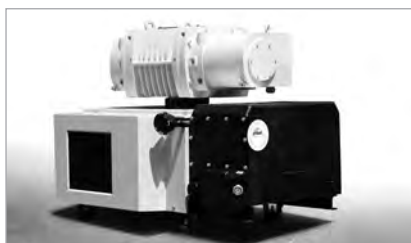
Pump system consisting of RUVAC WH 4400 and SOGEOVAC SV 630 B
